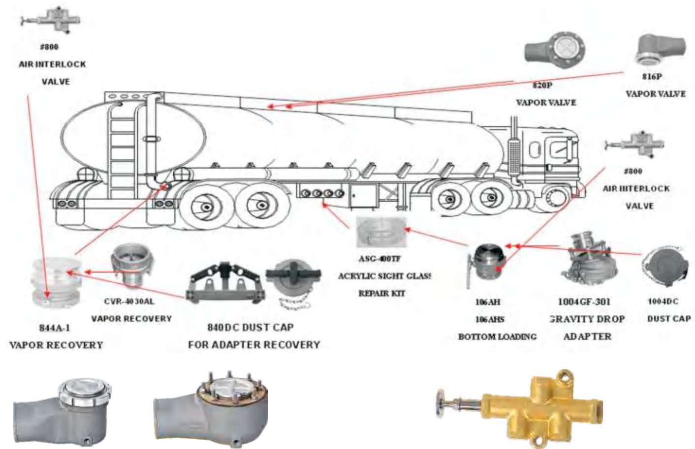
Pneumatic Air Interlock Valve A.P.I
